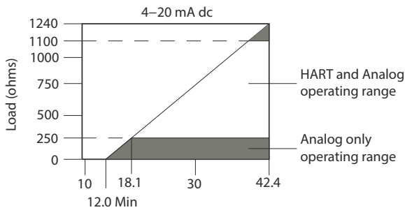
Figure 4: Load Limitations
